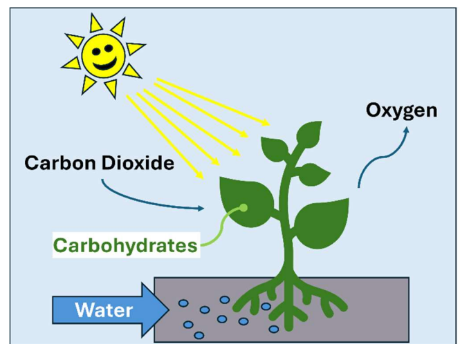
Figure 2 - Photosynthesis
