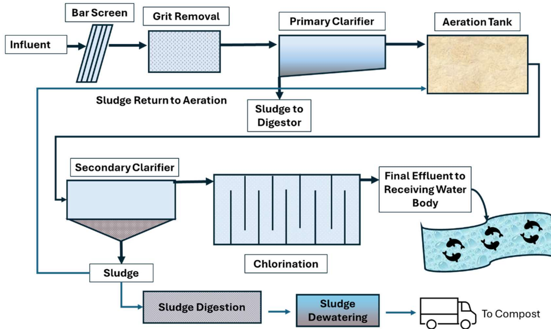
Figure 3 - Diagram of an Activated Sludge Wastewater Treatment Plant Process
